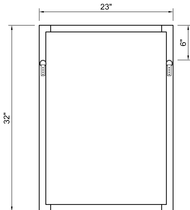
BACK VIEW
